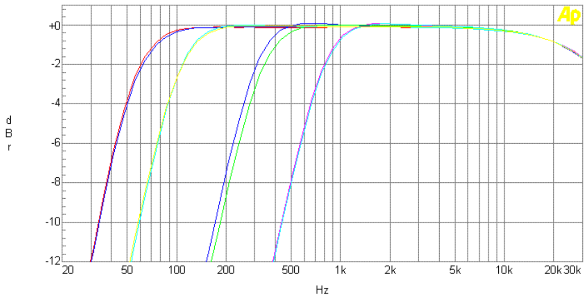
Chat 6. HPF Filter response
