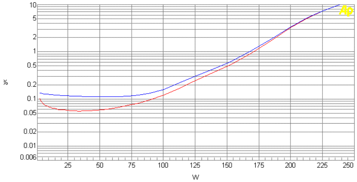
Chat 1. RMS output power @2ohm with THD+N
