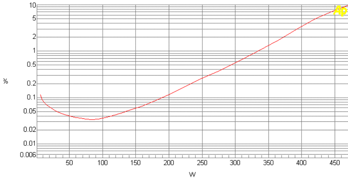
Chat 3. Bridged RMS power @4ohm with THD+N
