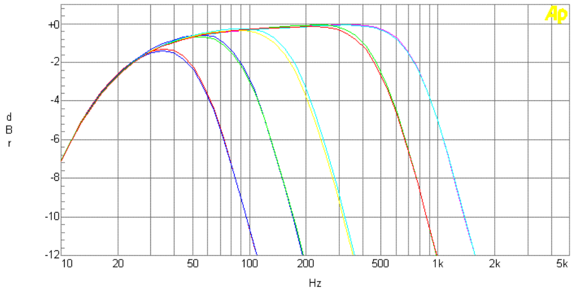
Chat 5. LPF response
