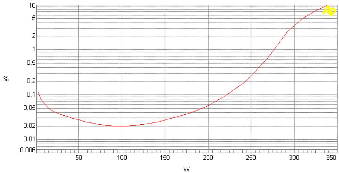
Chat 2. Bridged RMS power @8ohm with THD+N
