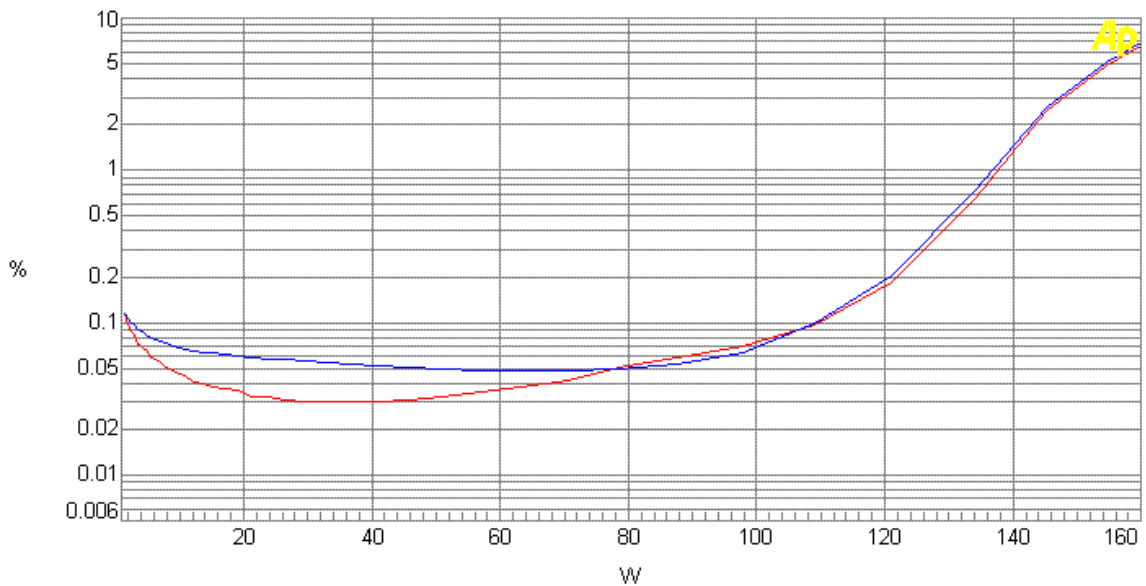
Chat 0. RMS output power @4ohm with THD+N
