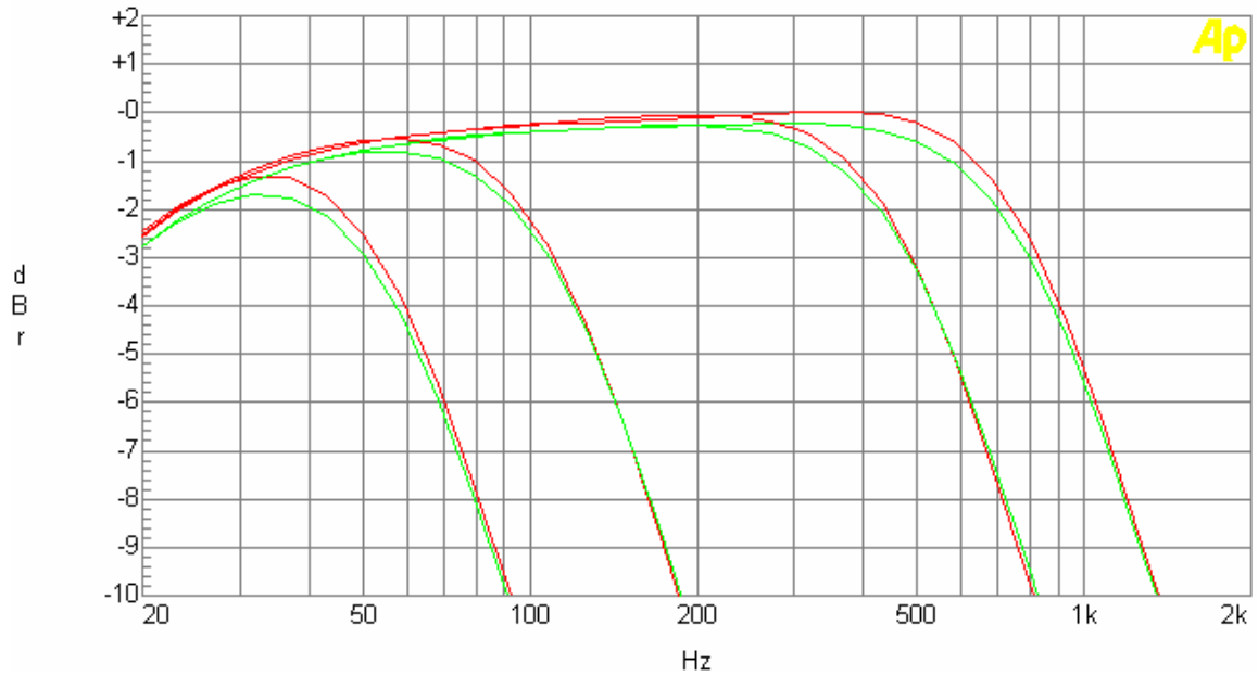
Chart 6. LPF response
