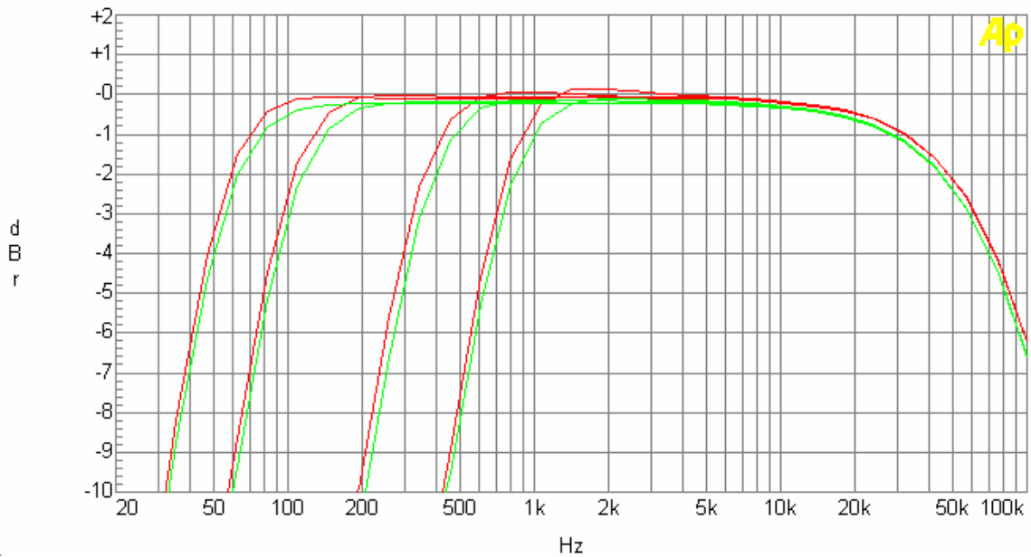
Chart 7. HPF Filter response
