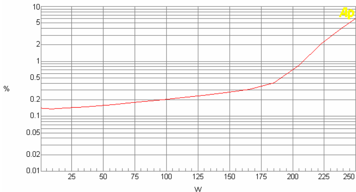
Chart 4. Bridged RMS power @4ohm with THD+N
