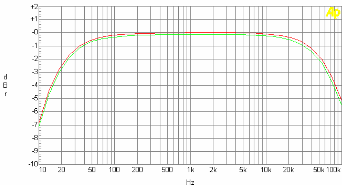
Chart 5. Frequency Response
