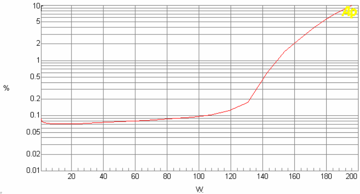
Chart 3. Bridged RMS power @8ohm with THD+N
