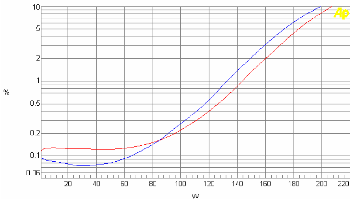
Chat 2. RMS output power @2ohm with THD+N
