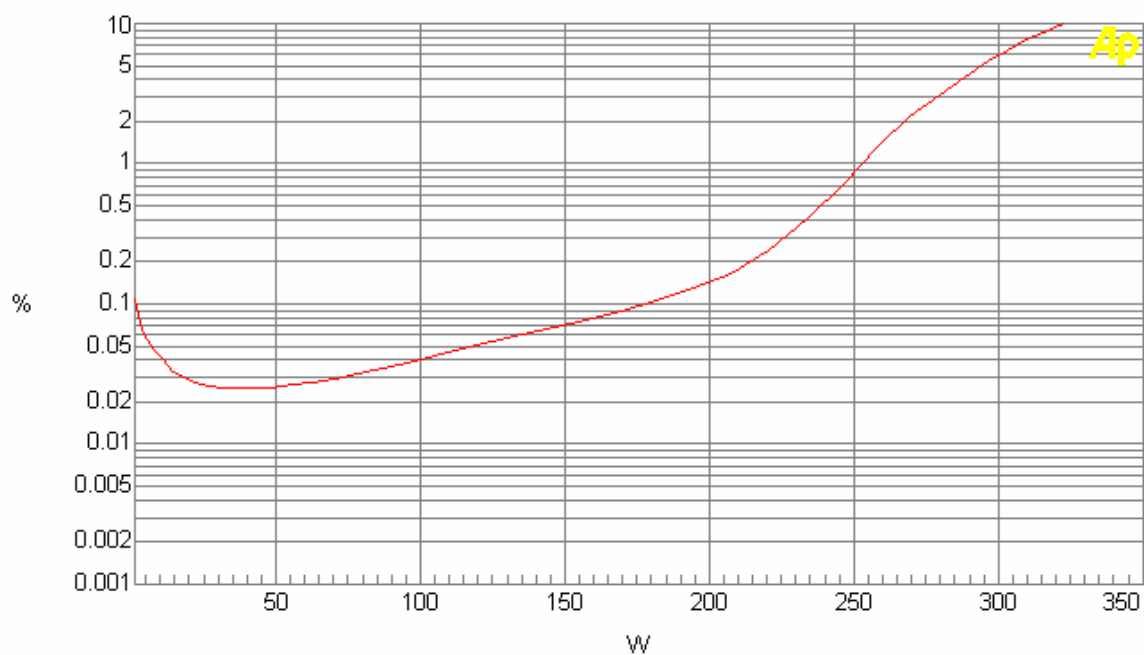
Chat 3. Bridged RMS power @8ohm with THD+N
