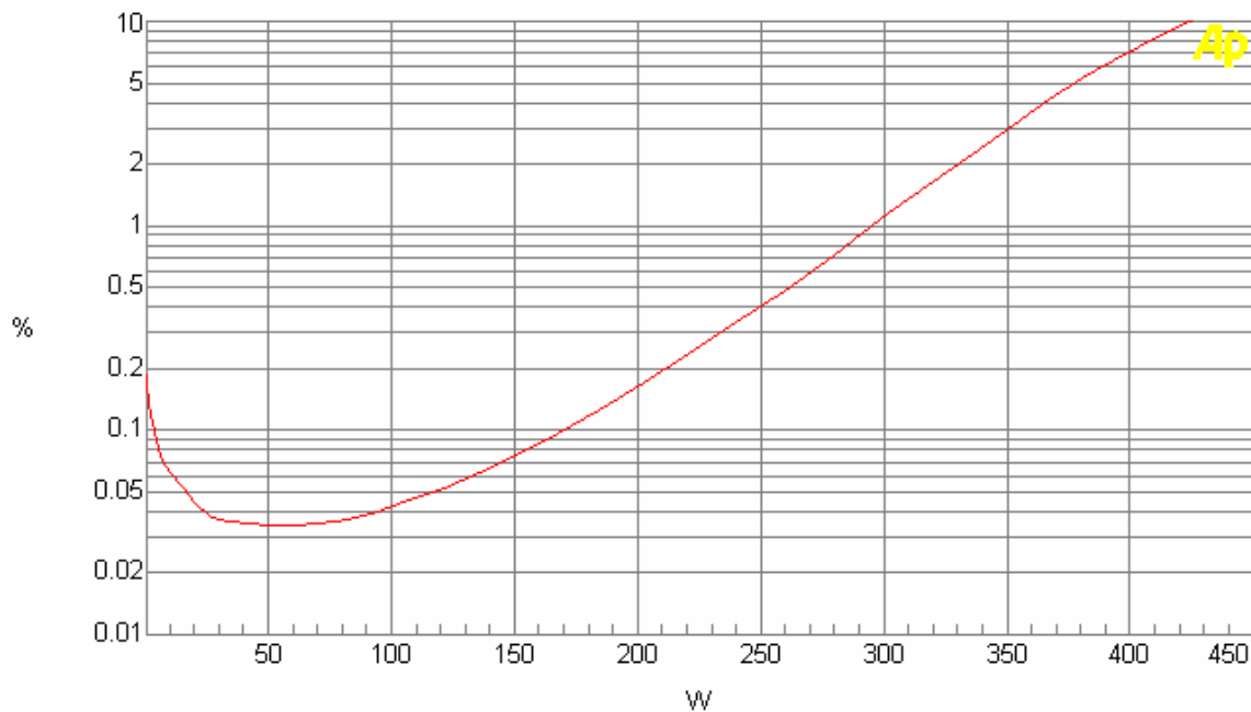
Chat 4. Bridged RMS power @4ohm with THD+N
