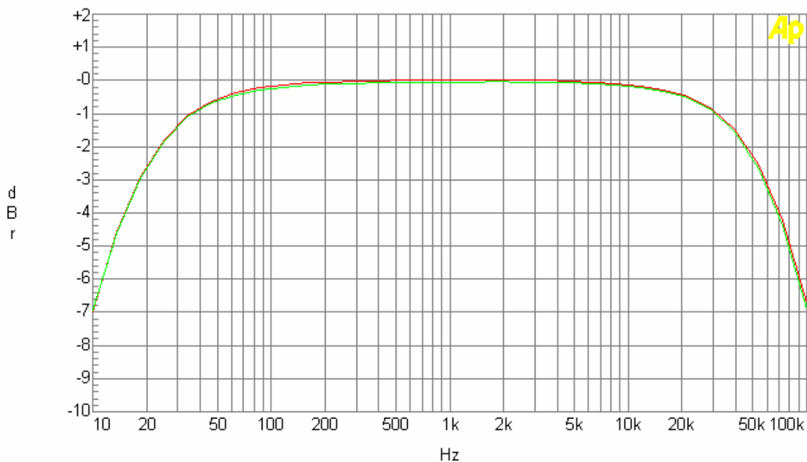
Chat 5. Frequency Response
