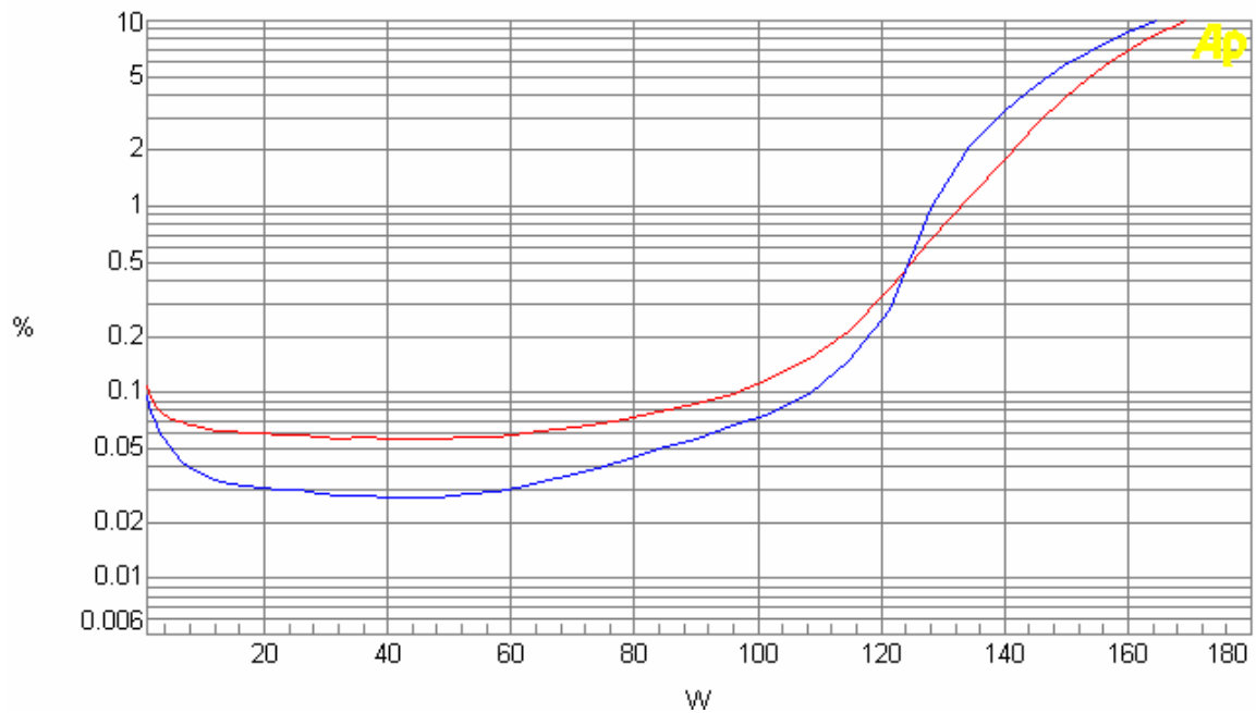
Chat 1. RMS output power @4ohm with THD+N
